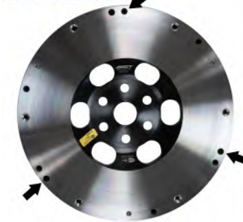
MZ027 = 8mm dowels
