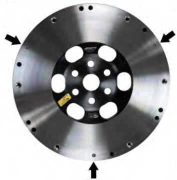
MZ027 = 8mm dowels
